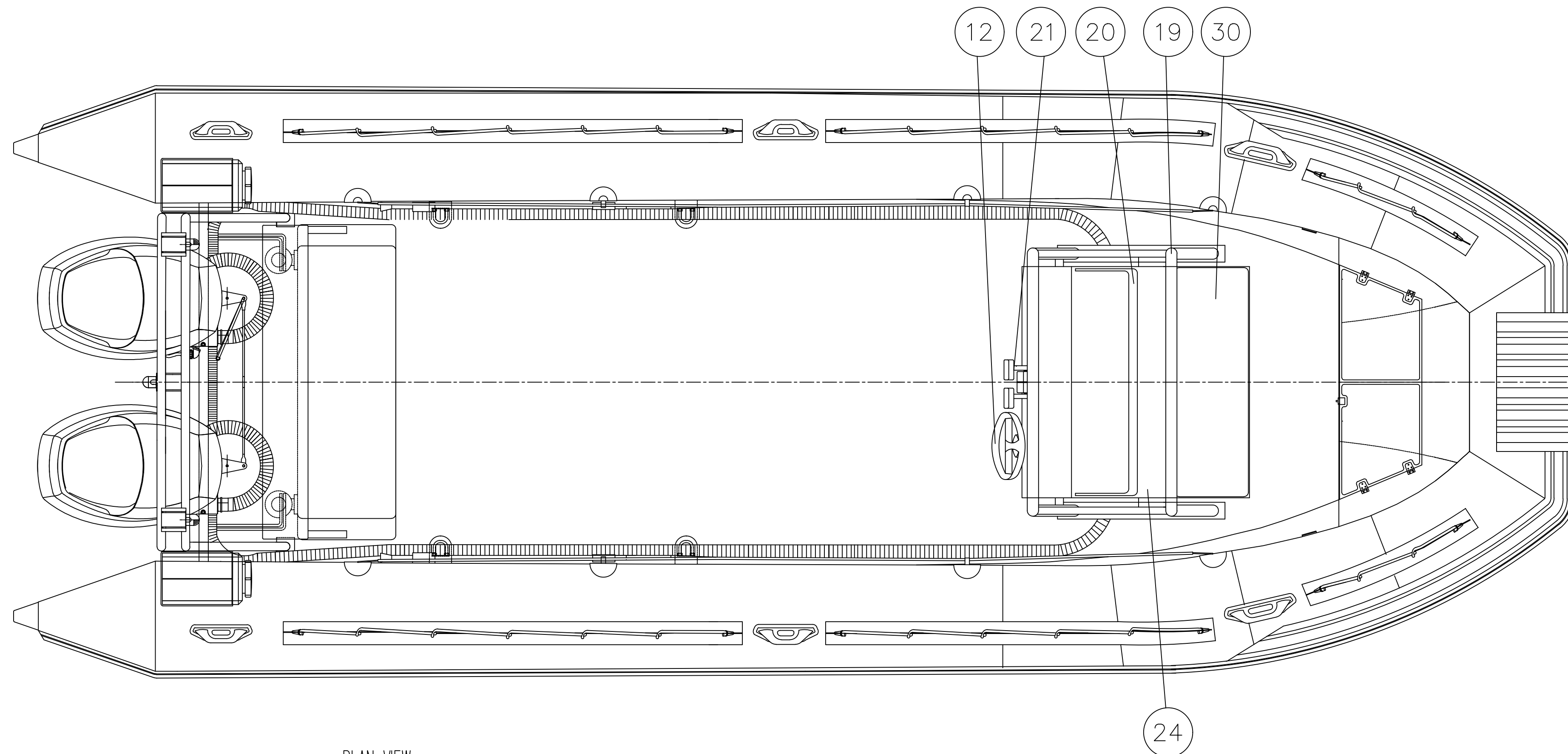
PLAN VIEW WITHOUT BIMINI
