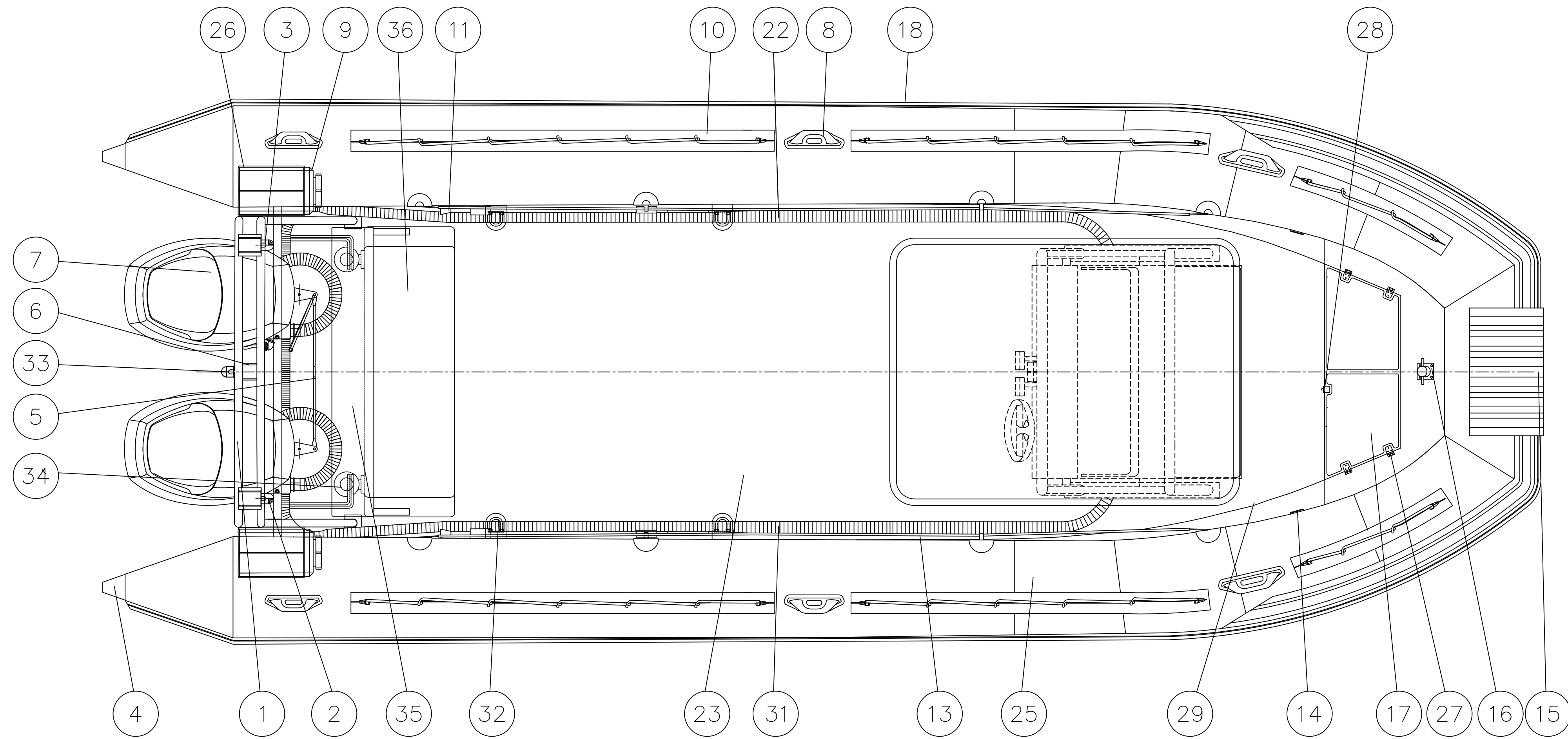
PLAN VIEW WITH BIMINI
